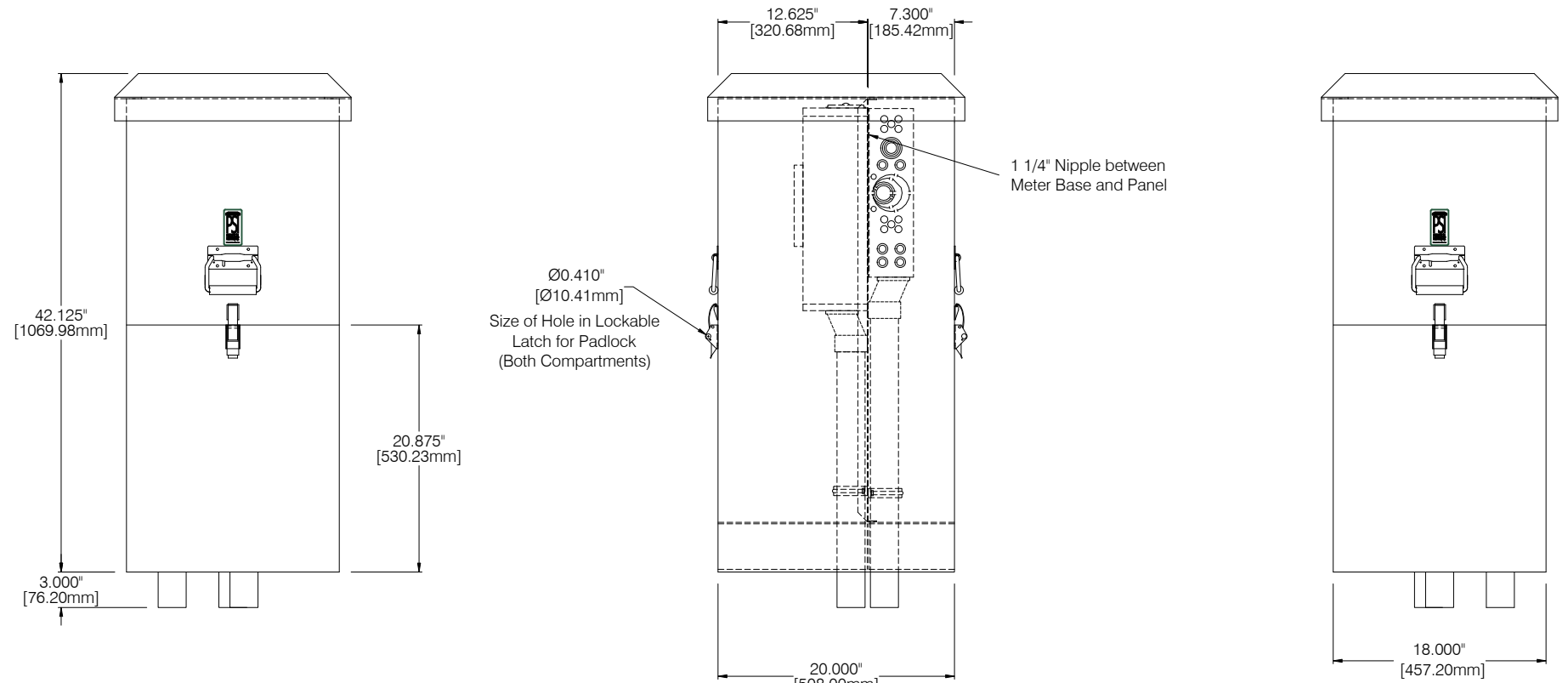
Meterbase Compartment Outside View with Panel in place
