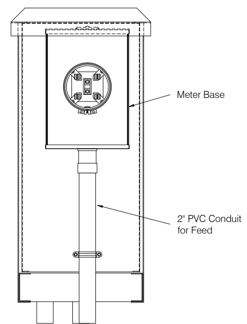
Meterbase Compartment Outside View with Panel Removed
