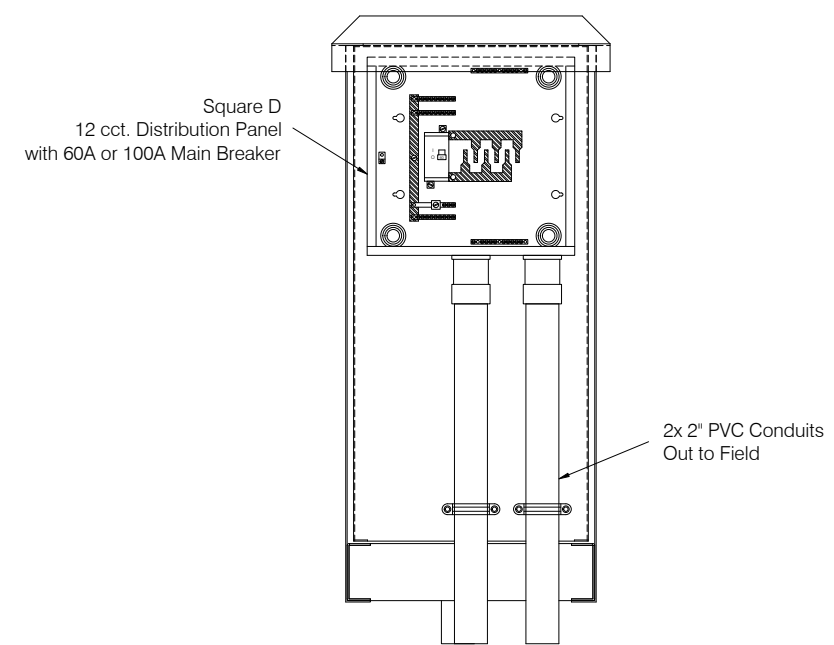
Distribution Panel Compartment Outside View with Panel Removed
