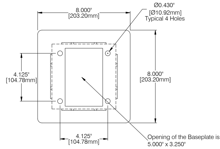
Baseplate (Magnified 2x)
