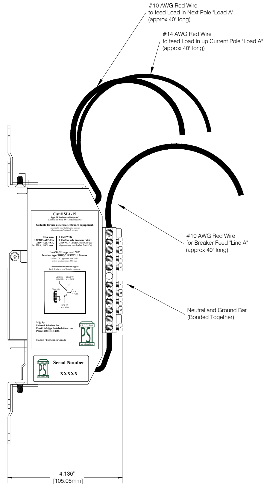
Side View with Locking Cover in Place
