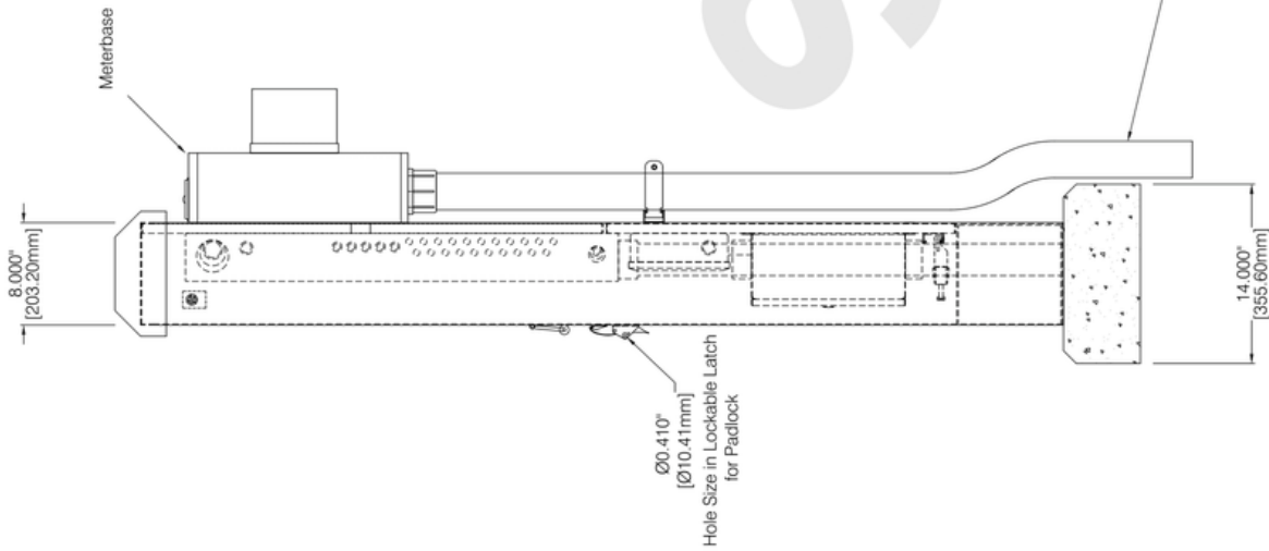
Side View with Front Covers Installed
