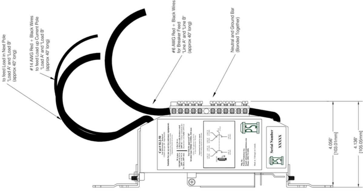
Side View with Locking Cover in Place
