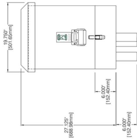
Meterbase Compartment Outside View with Panels in place
