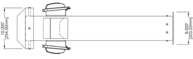
Front Outside View
