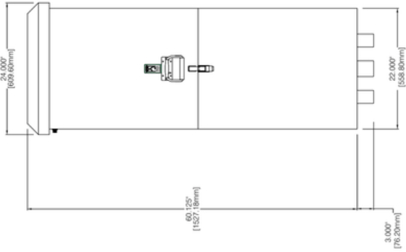
Meterbase Compartment Exterior View with Panels in place
